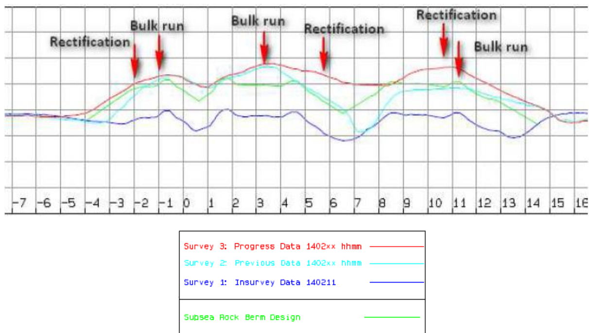
Figure 6 As-Built Cross Section of Rock Installation, Final Profile
