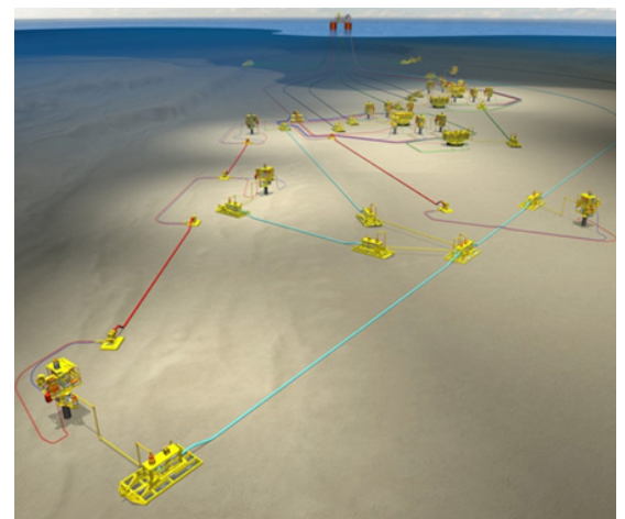
Innovator of subsea development: 2 six-slot drill centers with in-well gas lift and high-pressure water injection
