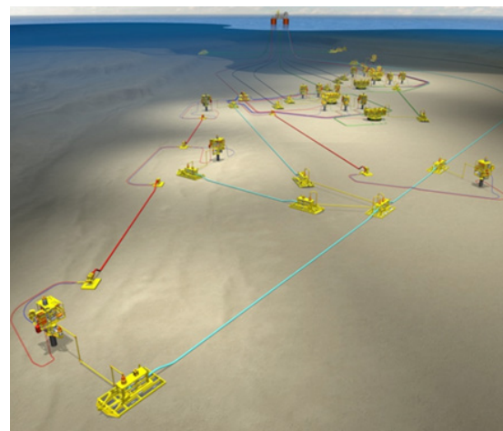
Innovator of subsea development: 2 six-slot drill centers with in-well gas lift and high pressure water injection
